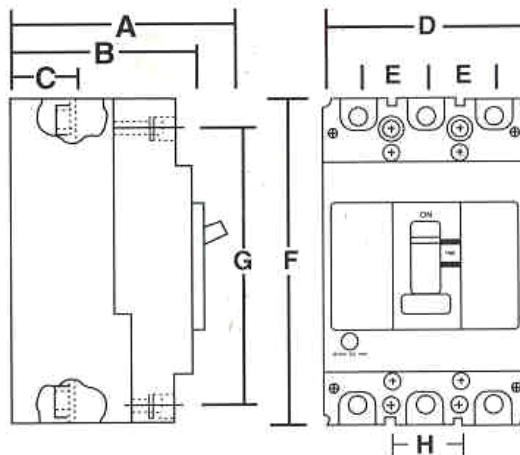
Dimensions(mm)
