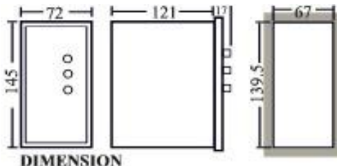
DIMENSION
